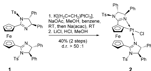
Scheme 1. Formation of the strained complex 2 by diastereoselective cycloplatination.
