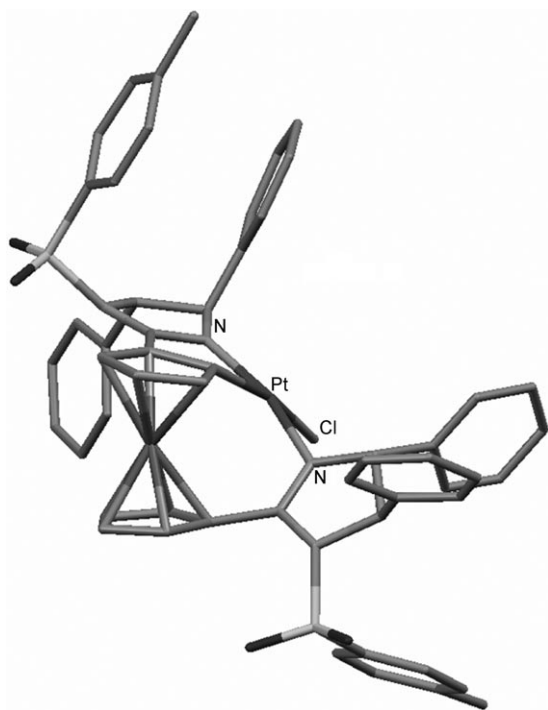
Figure 1. X-ray crystal structure of the strained platinacycle 2 .
