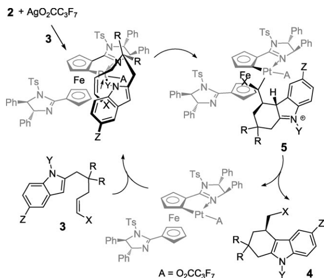
Scheme 2. Proposed mechanism for the intramolecular Friedel–Crafts alkylation of indoles.
